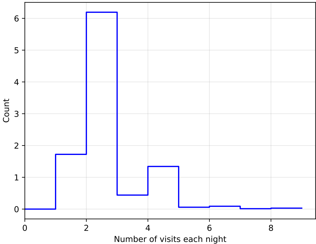
ddf_acor_sf15_lsf20_lsr20_v3.4_10yrs All sky: NVisitsPerNight 1e6
