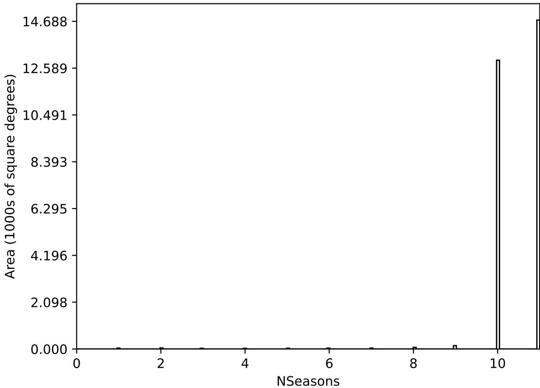
ddf_acor_sf15_lsf20_lsr20_v3.4_10yrs All sky all bands: NSeasons
