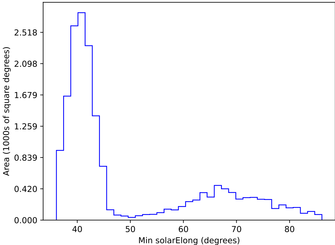
ddf_acor_sf15_lsf20_lsr20_v3.4_10yrs WFD z band: Min solarElong
