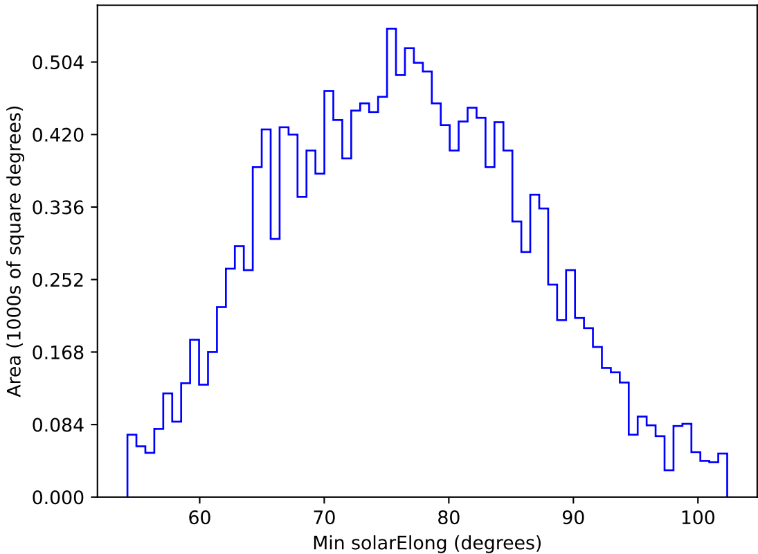
ddf_acor_sf15_lsf20_lsr20_v3.4_10yrs WFD u band: Min solarElong
