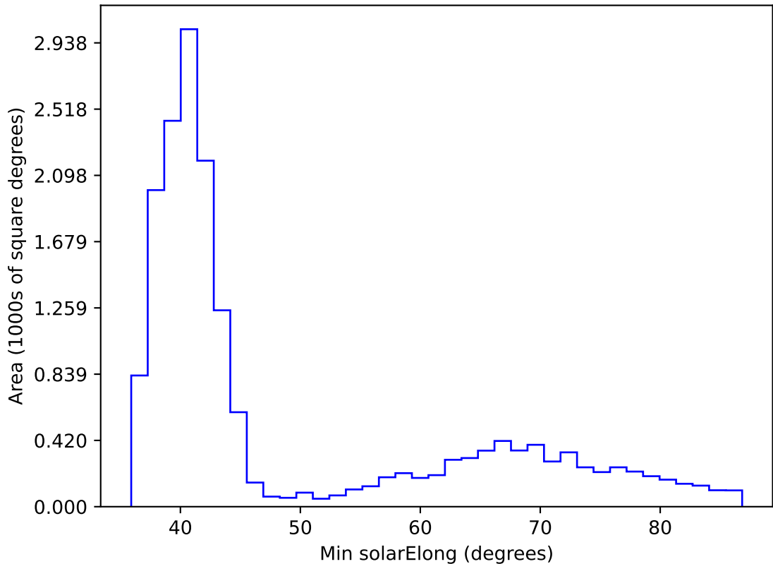
ddf_acor_sf15_lsf20_lsr20_v3.4_10yrs WFD i band: Min solarElong
