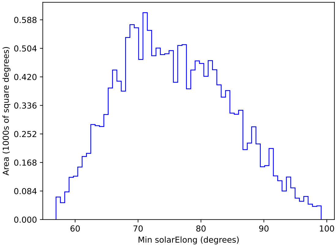
ddf_acor_sf15_lsf20_lsr20_v3.4_10yrs WFD g band: Min solarElong
