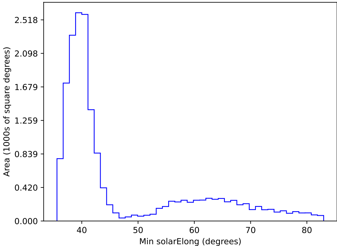
ddf_acor_sf15_lsf20_lsr20_v3.4_10yrs WFD all bands: Min solarElong
