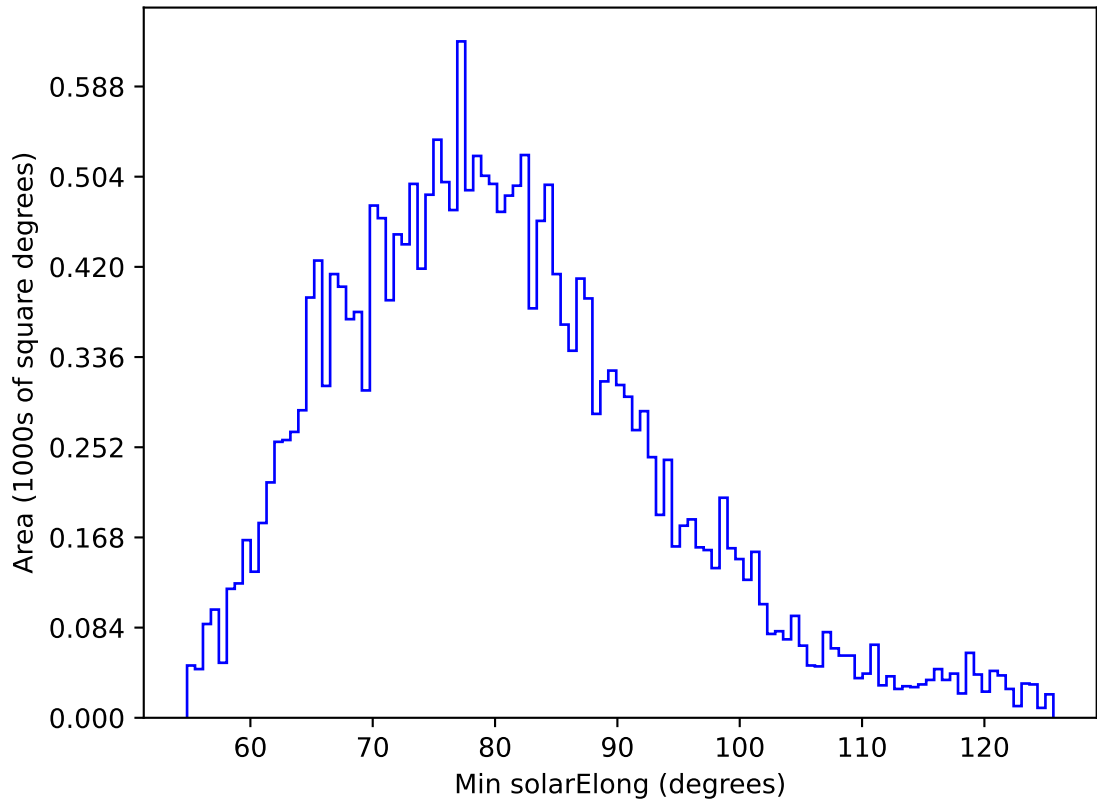
ddf_acor_sf15_lsf20_lsr20_v3.4_10yrs All sky u band: Min solarElong
