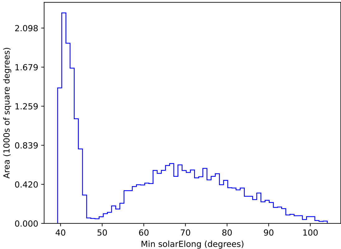
ddf_acor_sf15_lsf20_lsr20_v3.4_10yrs All sky r band: Min solarElong
