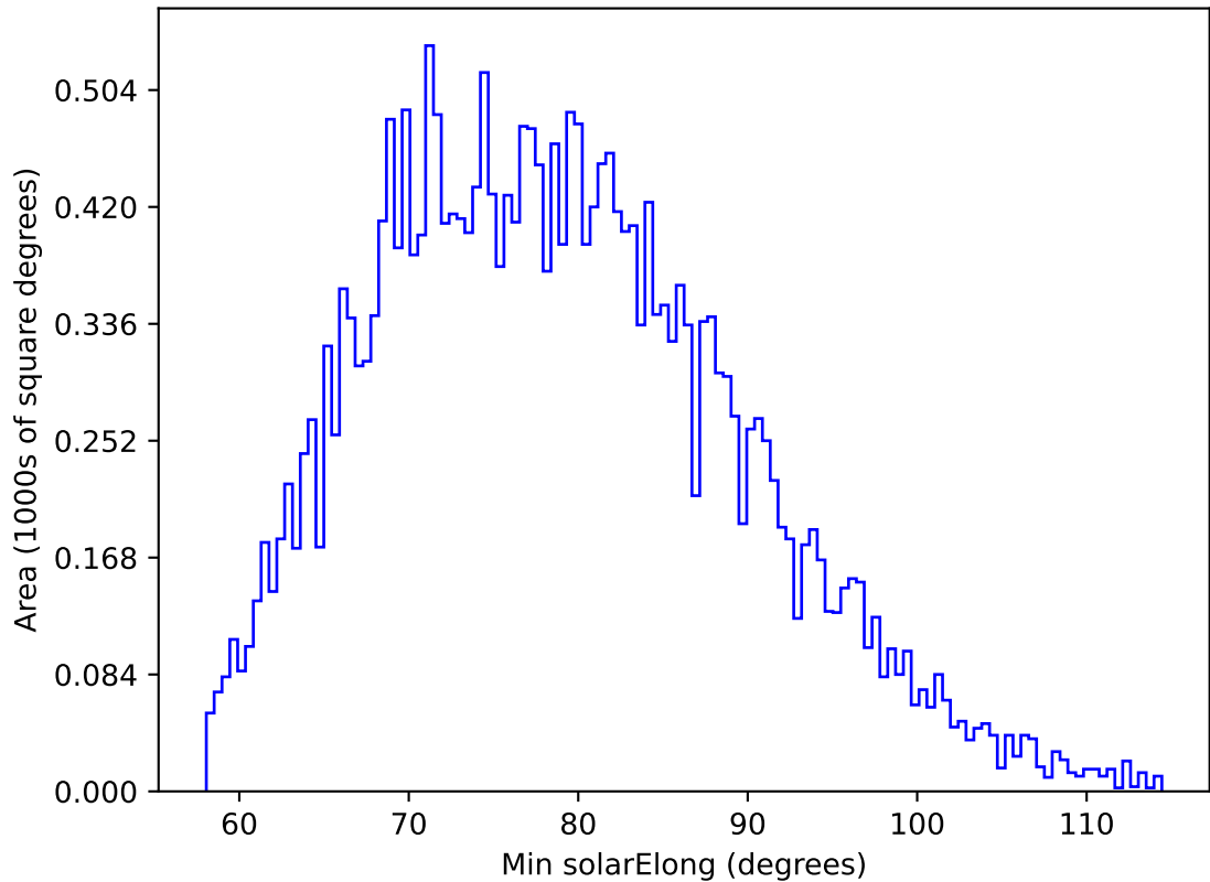
ddf_acor_sf15_lsf20_lsr20_v3.4_10yrs All sky g band: Min solarElong
