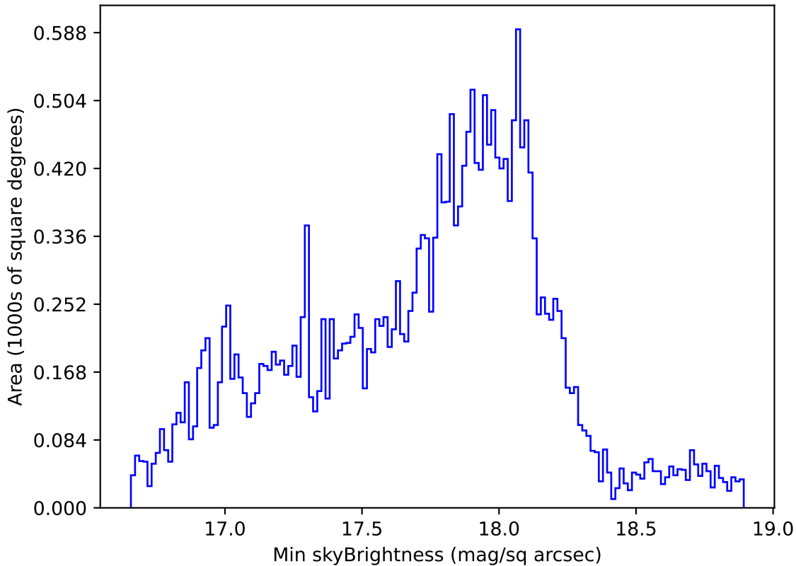
ddf_acor_sf15_lsf20_lsr20_v3.4_10yrs Yr 1 all bands: Min skyBrightness
