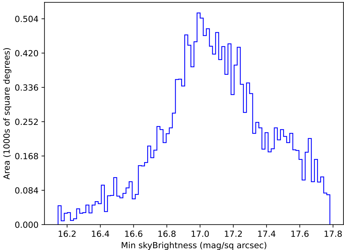
ddf_acor_sf15_lsf20_lsr20_v3.4_10yrs WFD y band: Min skyBrightness
