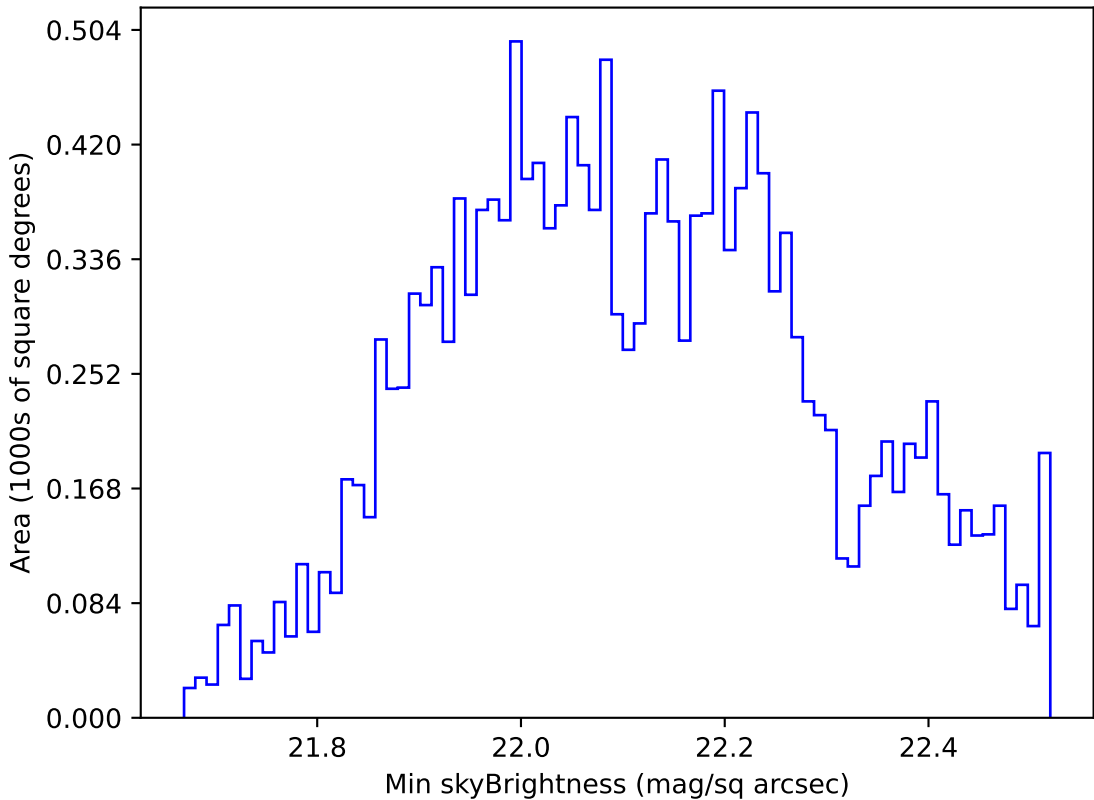
ddf_acor_sf15_lsf20_lsr20_v3.4_10yrs WFD u band: Min skyBrightness
