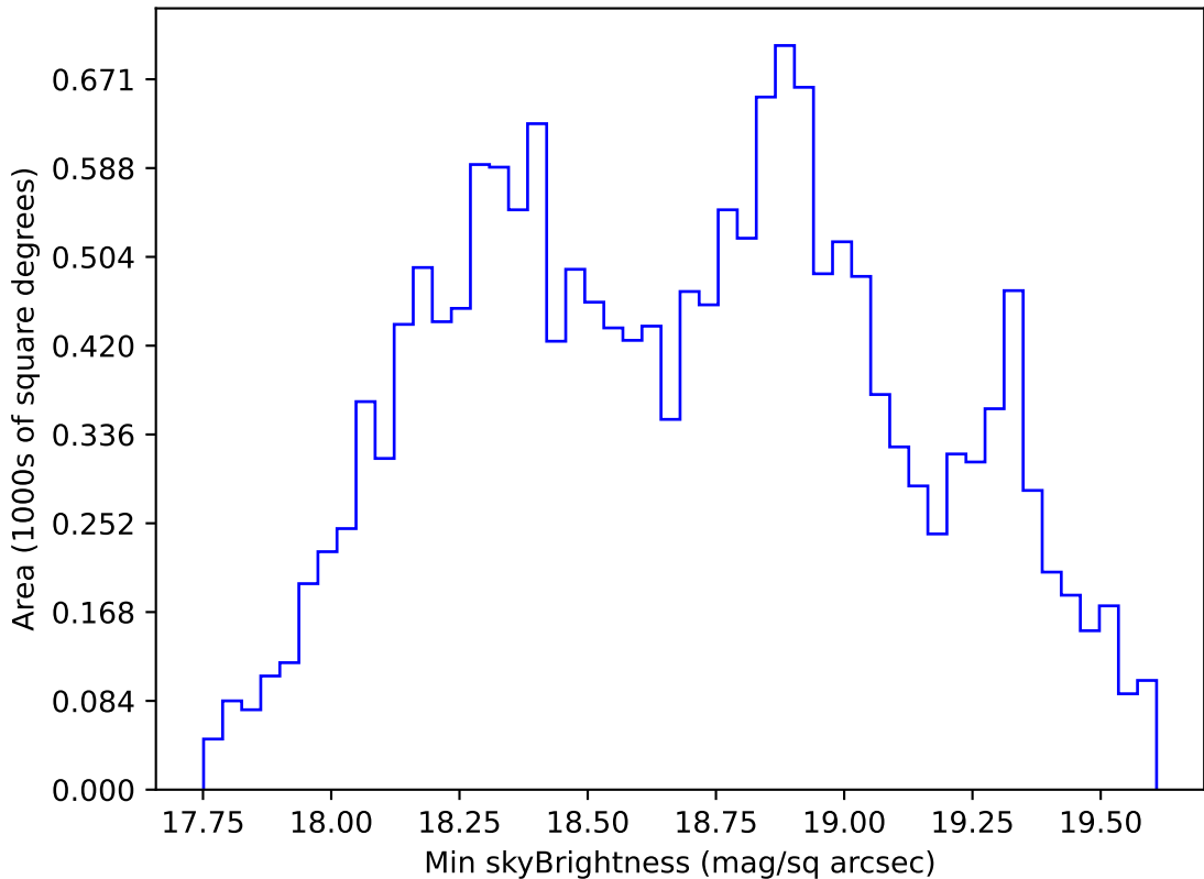
ddf_acor_sf15_lsf20_lsr20_v3.4_10yrs WFD r band: Min skyBrightness
