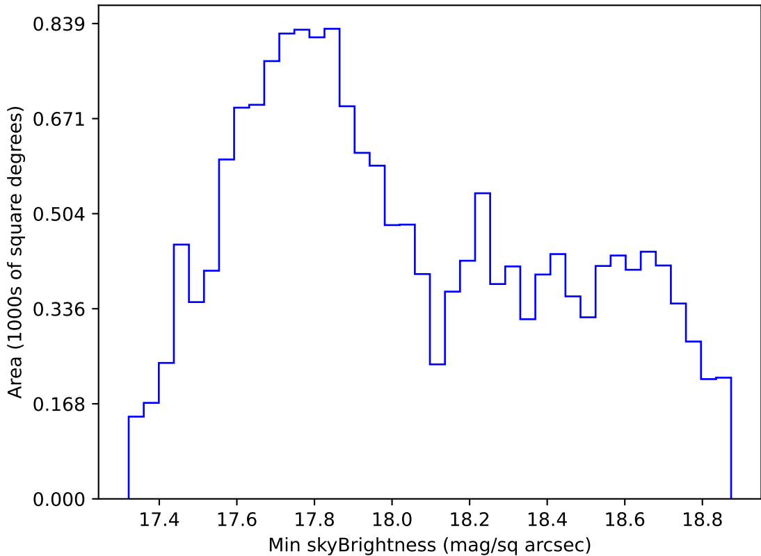
ddf_acor_sf15_lsf20_lsr20_v3.4_10yrs WFD i band: Min skyBrightness
