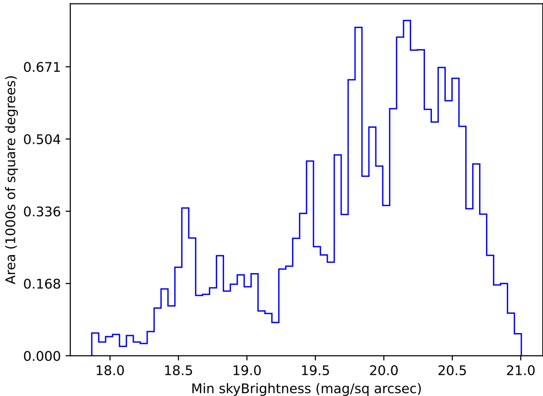
ddf_acor_sf15_lsf20_lsr20_v3.4_10yrs WFD g band: Min skyBrightness
