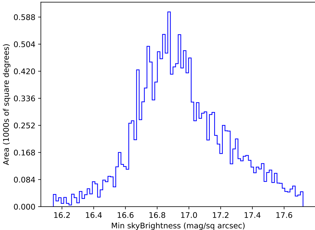
ddf_acor_sf15_lsf20_lsr20_v3.4_10yrs WFD all bands: Min skyBrightness
