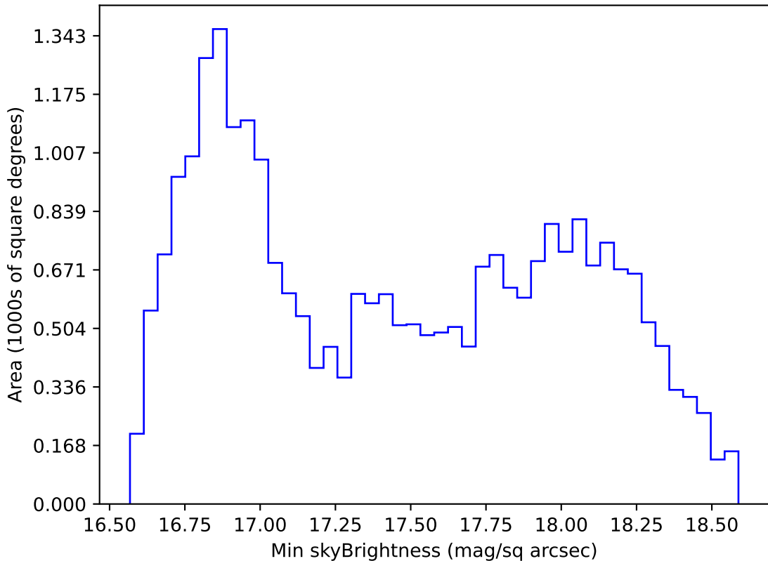
ddf_acor_sf15_lsf20_lsr20_v3.4_10yrs All sky z band: Min skyBrightness
