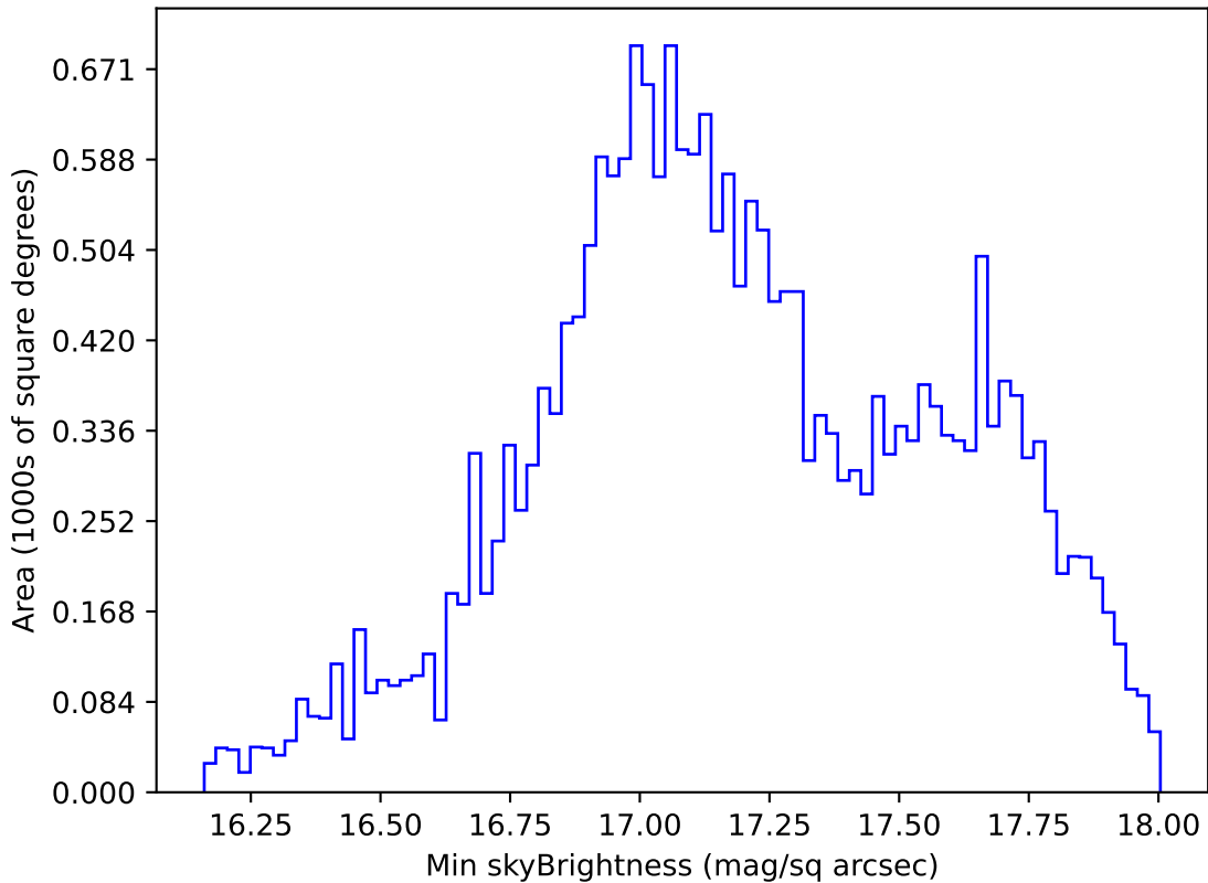
ddf_acor_sf15_lsf20_lsr20_v3.4_10yrs All sky y band: Min skyBrightness
