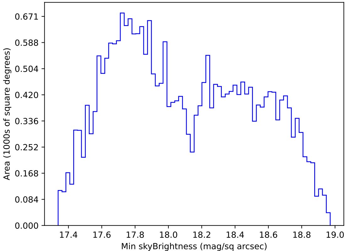
ddf_acor_sf15_ls20_lsr20_v3.4_10yrs All sky i band: Min skyBrightness
