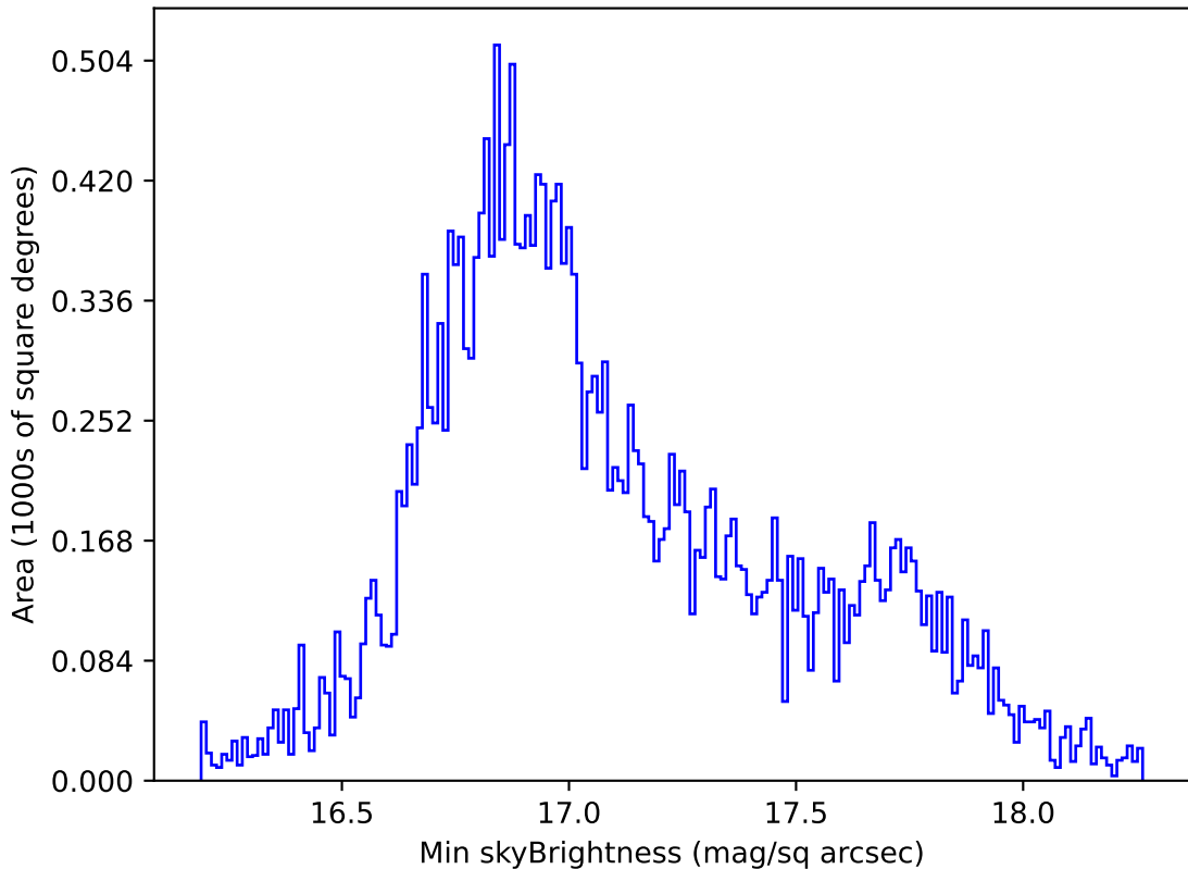
ddf_acor_sf15_lsf20_lsr20_v3.4_10yrs All sky all bands: Min skyBrightness
