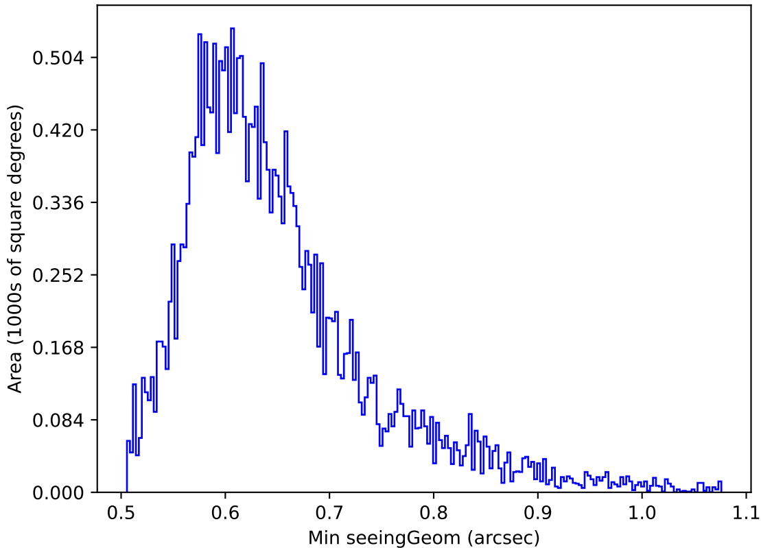
ddf_acor_sf15_lsf20_lsr20_v3.4_10yrs Yr 1 z band: Min seeingGeom
