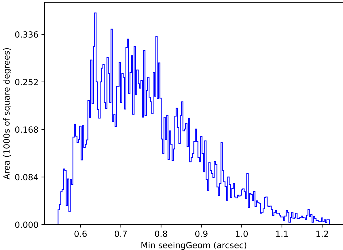
ddf_acor_sf15_lsf20_lsr20_v3.4_10yrs Yr 1 u band: Min seeingGeom
