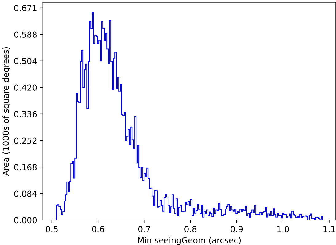
ddf_acor_sf15_lsf20_lsr20_v3.4_10yrs Yr 1 r band: Min seeingGeom
