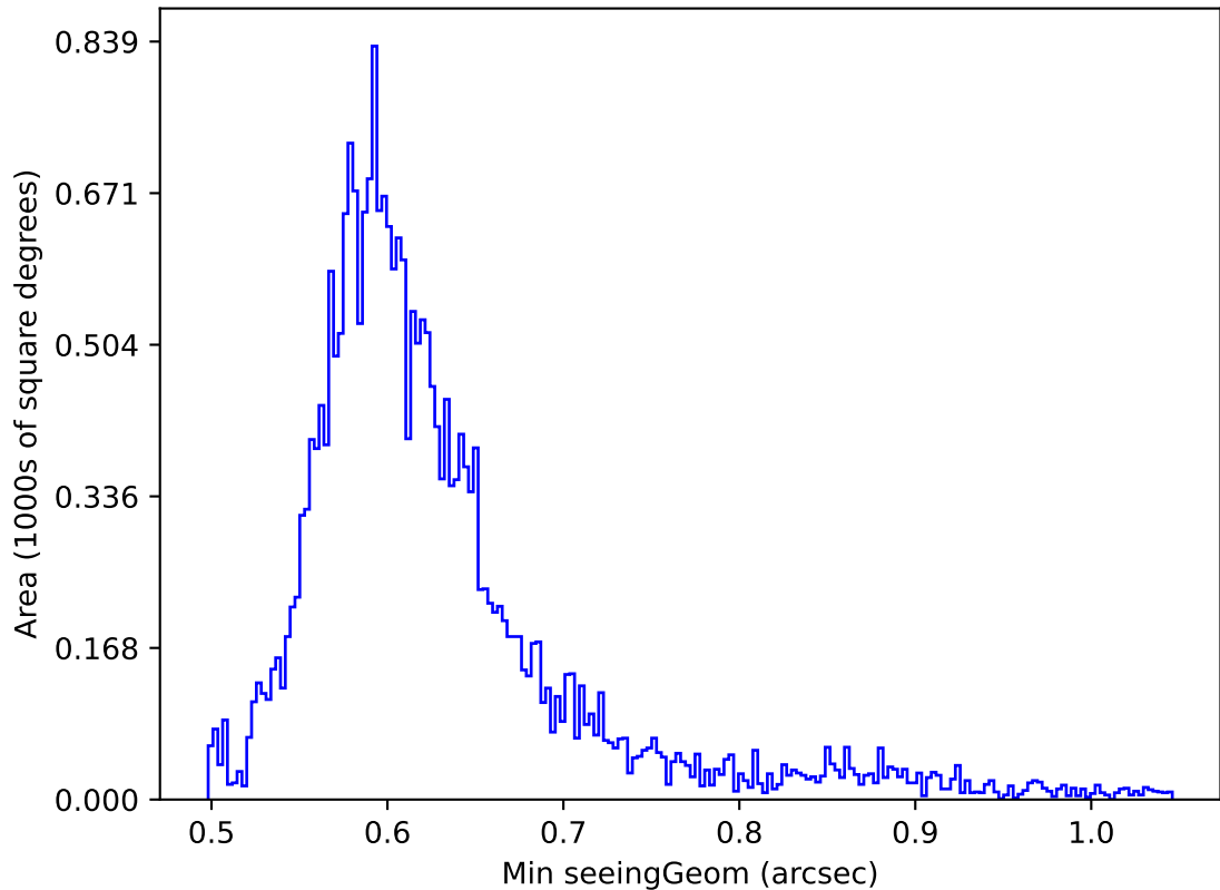
ddf_acor_sf15_lsf20_lsr20_v3.4_10yrs Yr 1 i band: Min seeingGeom
