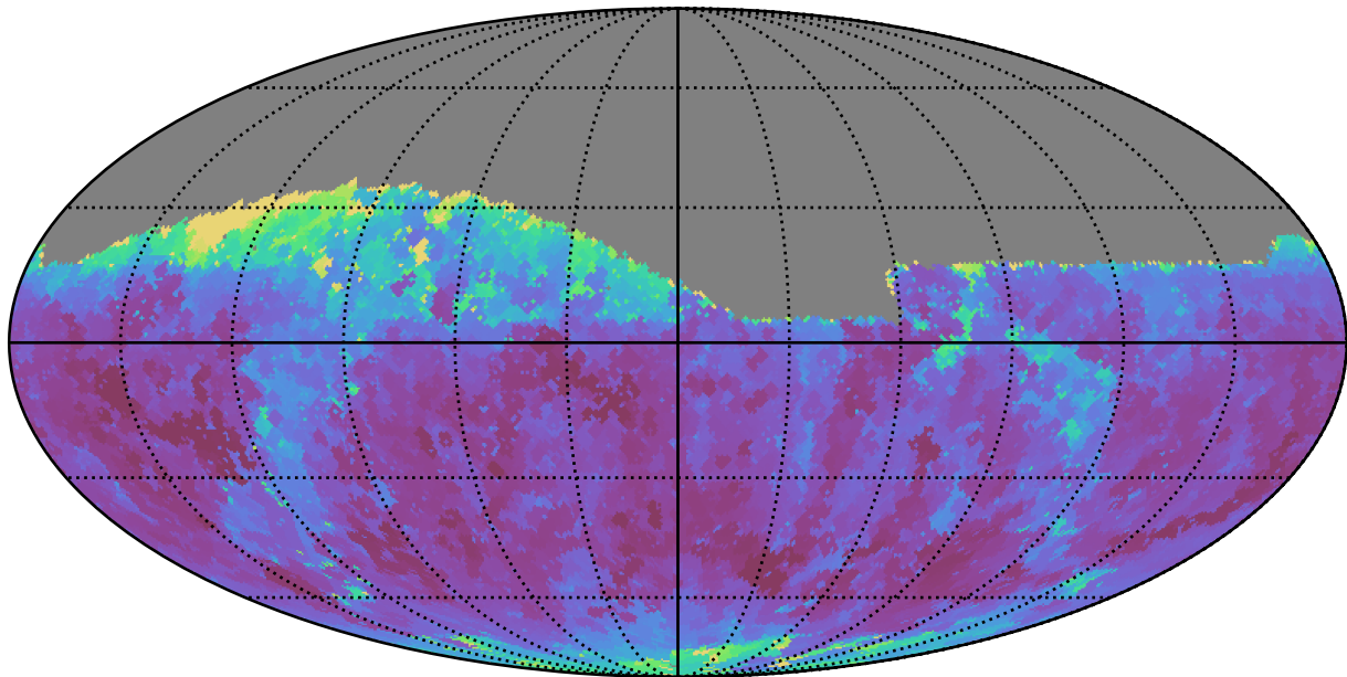
ddf_acor_sf15_lsf20_lsr20_v3.4_10yrs Yr 1 z band: Min seeingEff
