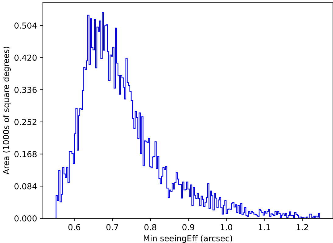
ddf_acor_sf15_ls20_lsr20_v3.4_10yrs Yr 1 z band: Min seeingEff
