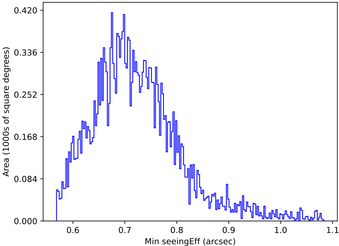
ddf_acor_sf15_ls20_lsr20_v3.4_10yrs Yr 1 y band: Min seeingEff
