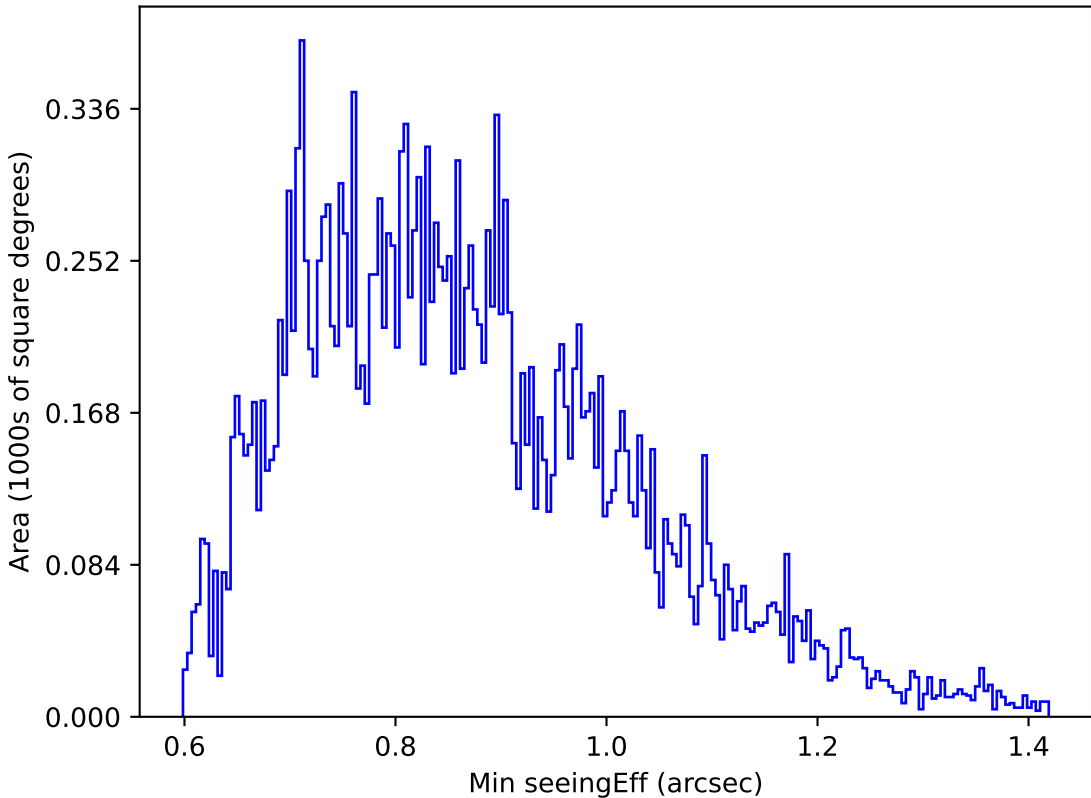
ddf_acor_sf15_lsf20_lsr20_v3.4_10yrs Yr 1 u band: Min seeingEff
