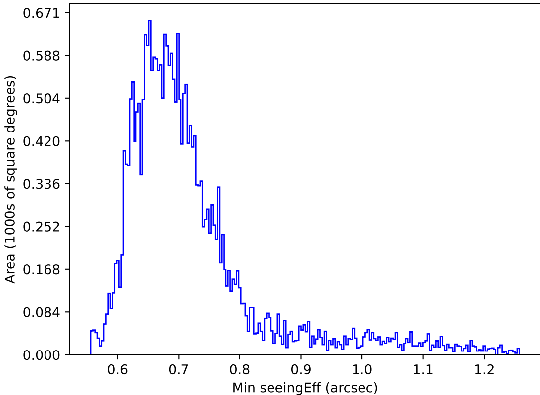
ddf_acor_sf15_lsf20_lsr20_v3.4_10yrs Yr 1 r band: Min seeingEff
