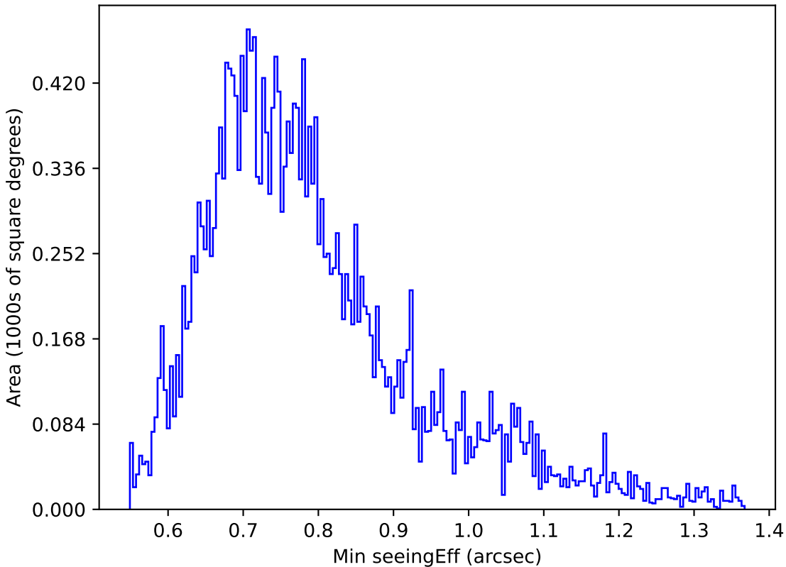
ddf_acor_sf15_lsf20_lsr20_v3.4_10yrs Yr 1 g band: Min seeingEff
