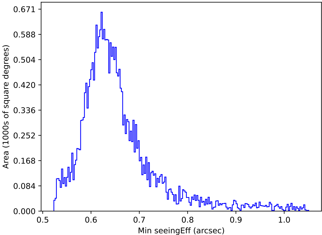
ddf_acor_sf15_lsf20_lsr20_v3.4_10yrs Yr 1 all bands: Min seeingEff
