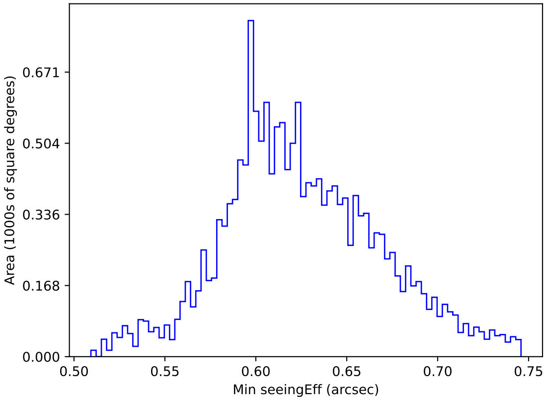
ddf_acor_sf15_lsf20_lsr20_v3.4_10yrs WFD y band: Min seeingEff
