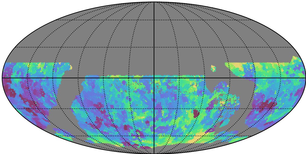
ddf_acor_sf15_lsf20_lsr20_v3.4_10yrs WFD u band: Min seeingEff
