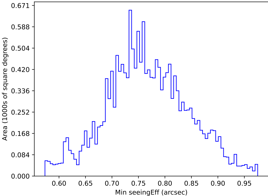
ddf_acor_sf15_lsf20_lsr20_v3.4_10yrs WFD u band: Min seeingEff
