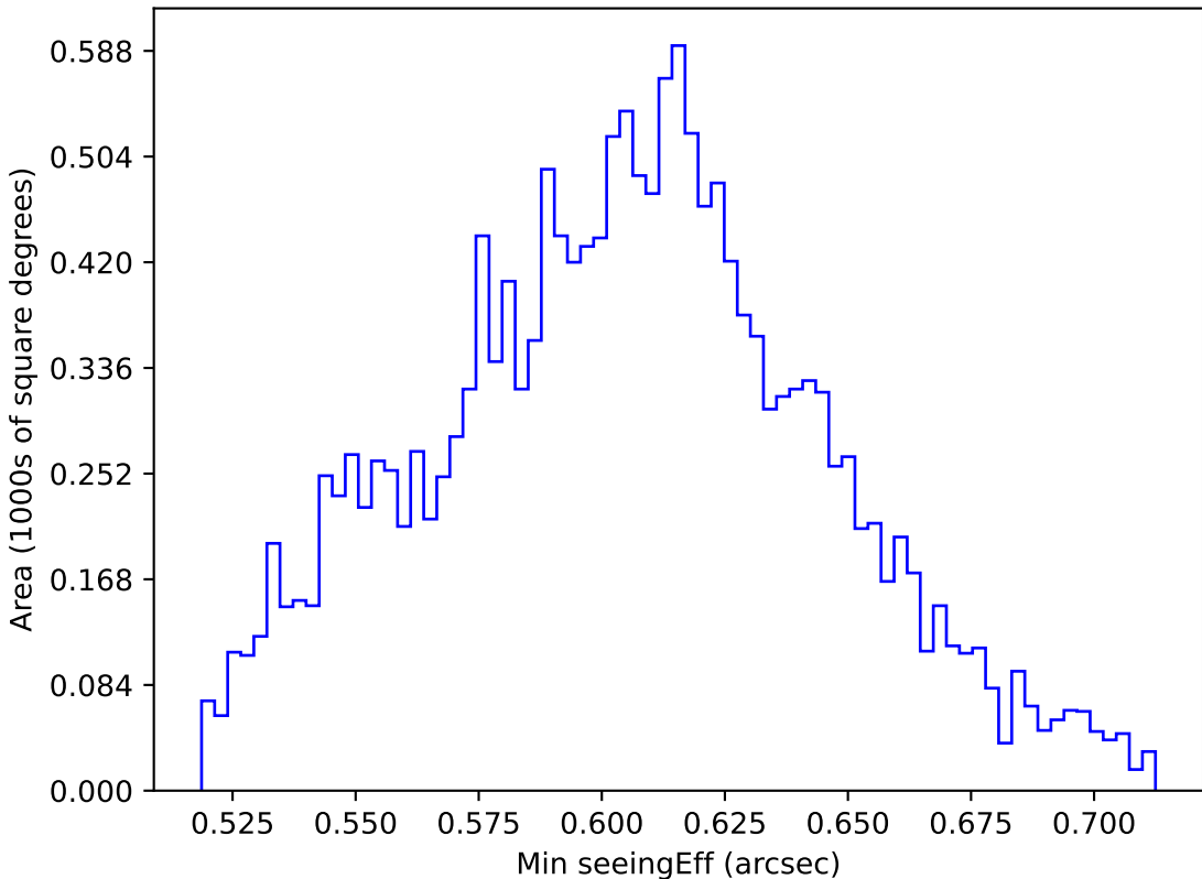
ddf_acor_sf15_lsf20_lsr20_v3.4_10yrs WFD i band: Min seeingEff
