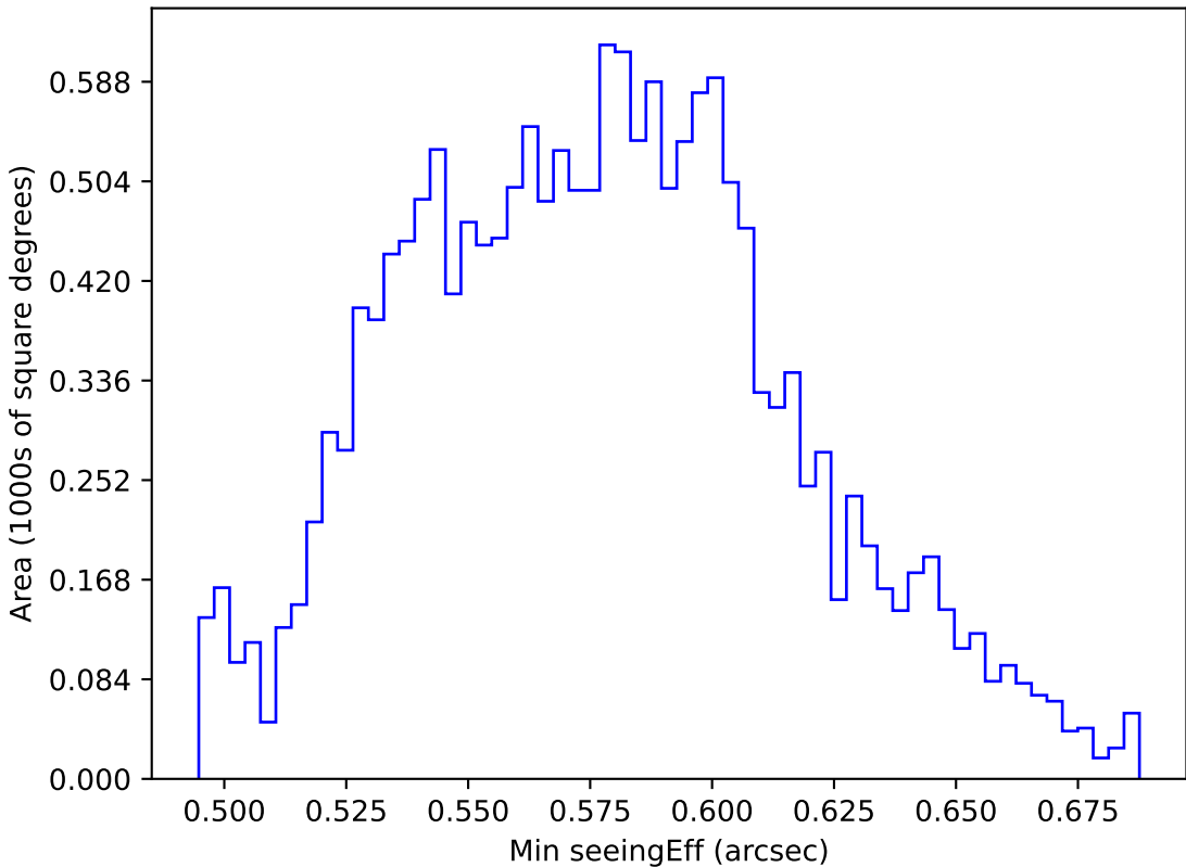
ddf_acor_sf15_lsf20_lsr20_v3.4_10yrs WFD all bands: Min seeingEff
