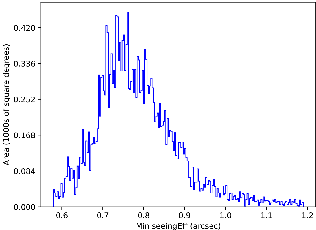
ddf_acor_sf15_lsf20_lsr20_v3.4_10yrs All sky u band: Min seeingEff
