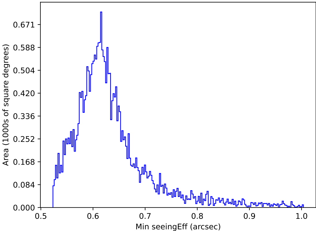
ddf_acor_sf15_lsf20_lsr20_v3.4_10yrs All sky i band: Min seeingEff
