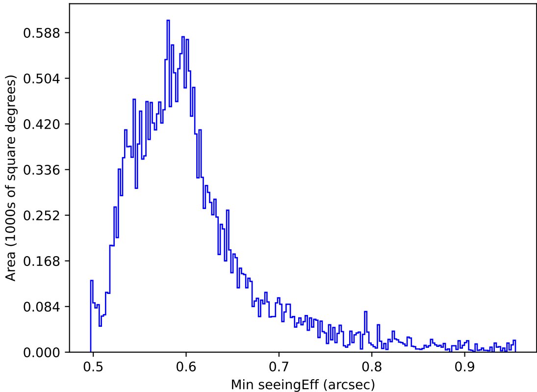
ddf_acor_sf15_lsf20_lsr20_v3.4_10yrs All sky all bands: Min seeingEff
