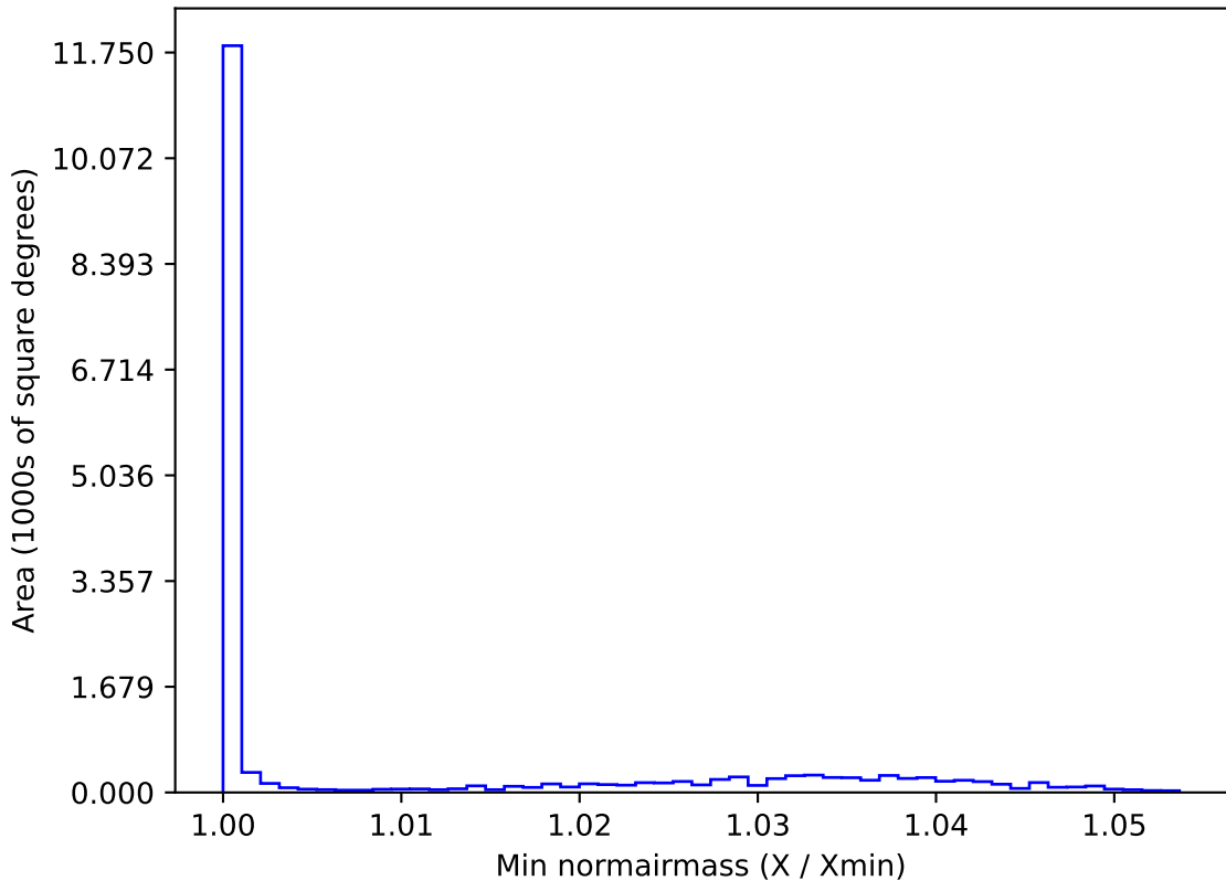
ddf_acor_sf15_lsf20_lsr20_v3.4_10yrs WFD u band: Min normairmass
