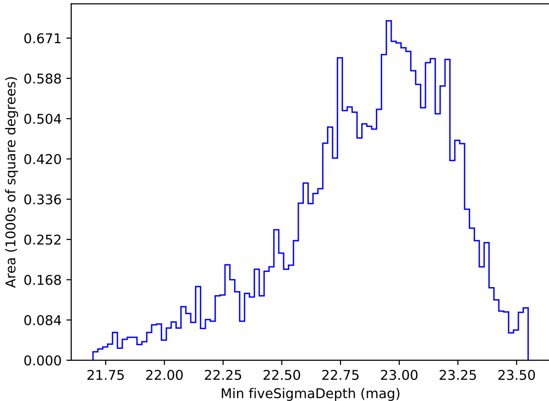
ddf_acor_sf15_lsf20_lsr20_v3.4_10yrs Yr 1 u band: Min fiveSigmaDepth
