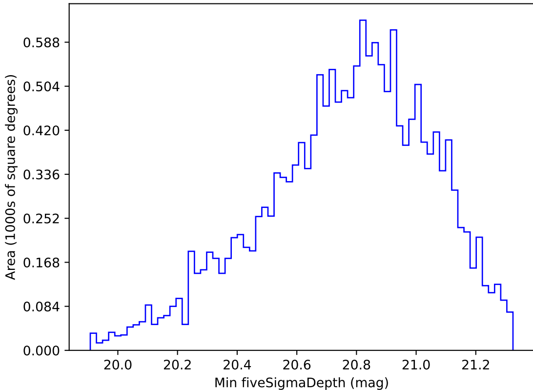
ddf_acor_sf15_lsf20_lsr20_v3.4_10yrs WFD all bands: Min fiveSigmaDepth
