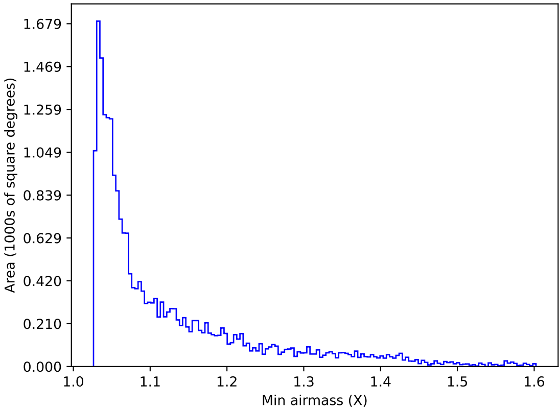
ddf_acor_sf15_lsf20_lsr20_v3.4_10yrs Yr 1 y band: Min airmass
