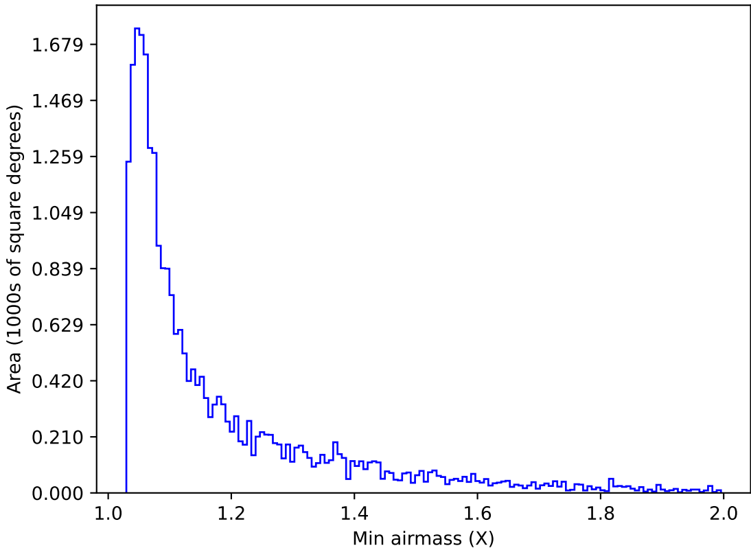
ddf_acor_sf15_lsf20_lsr20_v3.4_10yrs Yr 1 g band: Min airmass
