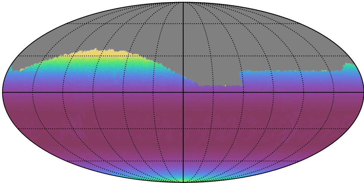
ddf_acor_sf15_lsf20_lsr20_v3.4_10yrs Yr 1 all bands: Min airmass
