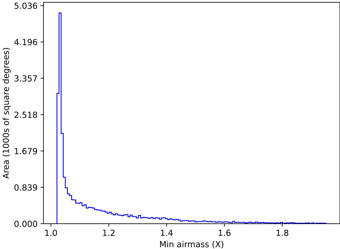
ddf_acor_sf15_lsf20_lsr20_v3.4_10yrs Yr 1 all bands: Min airmass
