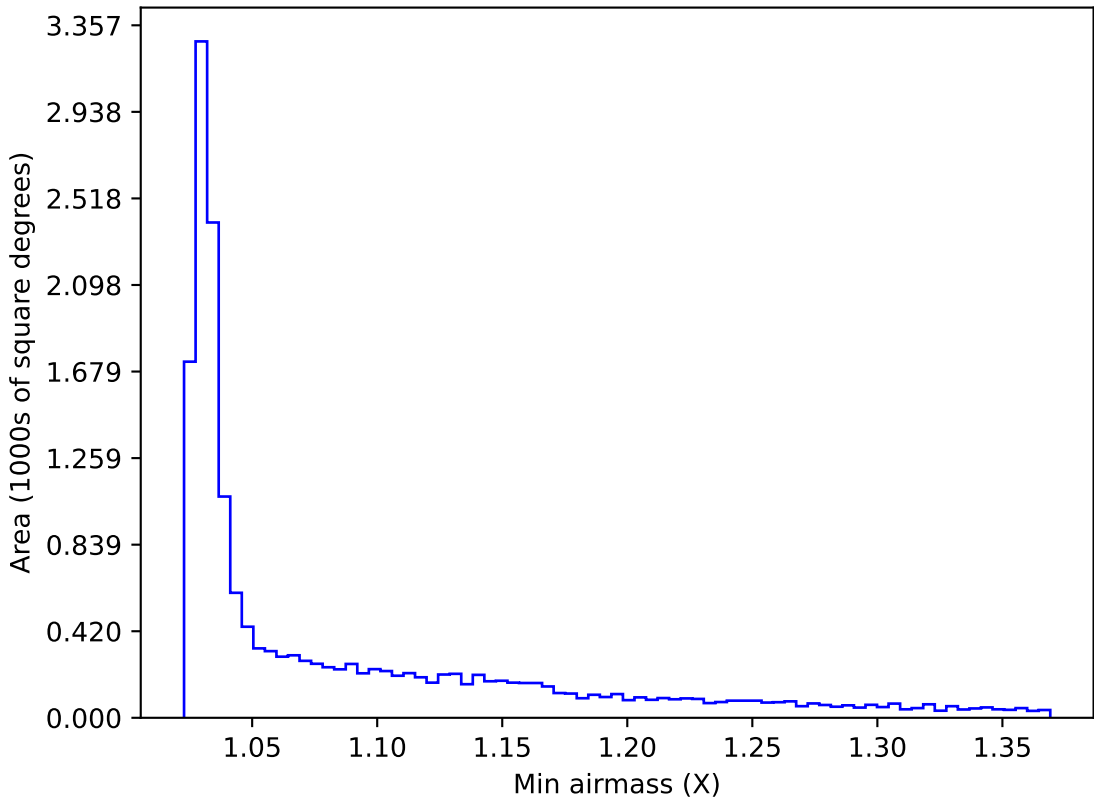
ddf_acor_sf15_lsf20_lsr20_v3.4_10yrs WFD y band: Min airmass
