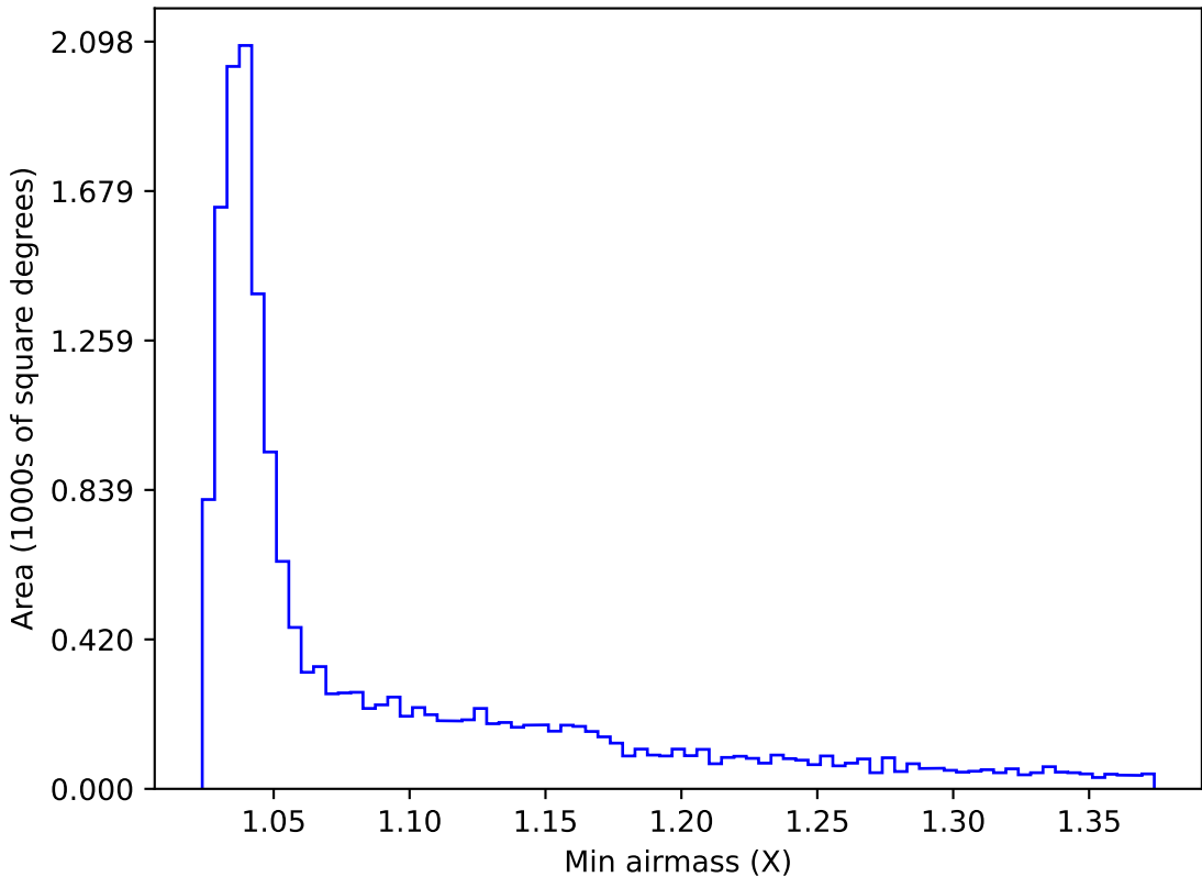
ddf_acor_sf15_lsf20_lsr20_v3.4_10yrs WFD u band: Min airmass
