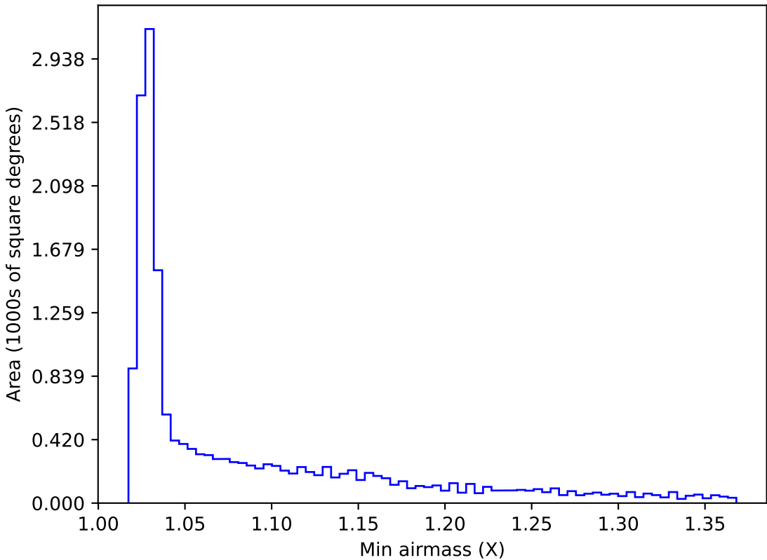
ddf_acor_sf15_lsf20_lsr20_v3.4_10yrs WFD i band: Min airmass
